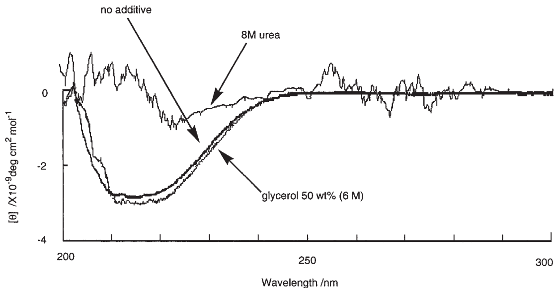
Figure 1. CD spectra of carboxypeptidase-Y in Tris-HCl buffer at pH 6.5 (no additive), in 50 wt% glycerol in Tris-HCl buffer at pH 6.5 and in 8 M urea in Tris-HCl buffer
