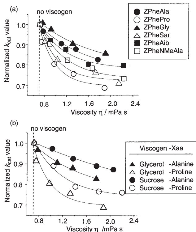
Figure 3. (a) Dependence of the k_{\text{cat}} of CPD-Y-catalysed hydrolysis of dipeptides Z-Phe-Xaa on viscosity in glycerol-Tris-HCl buffer mixed solvent. (b) Dependence of k_{\text{cat}} of the dipeptide Z-Phe-Xaa hydrolysis on viscosity with sucrose or glycerol as viscogen
